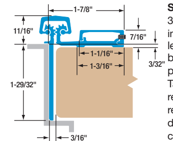
SL60 57" length. Hinge opens to 180°. SL62 57" length. Self-closing hinge opens to 120°.
