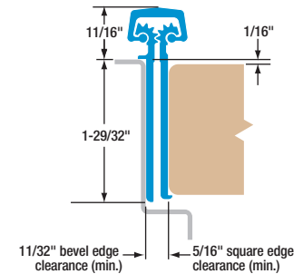
SL24 SD/HD/LL 1/16" door inset. Door edge protector. Frame leaf covers butt hinge preps.
