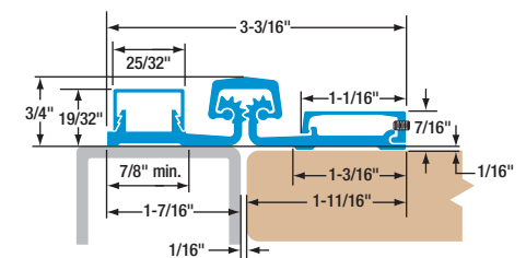
SL57 SD/HD 1/16" door inset. Frame leaf fits narrow (7/8") frame face. Tamper-resistant door leaf cover.
