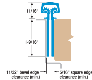
SL11 SD/HD/LL Flush mounted (no door inset).
